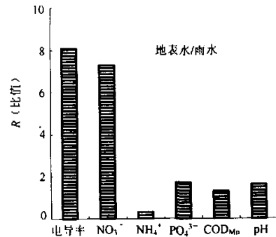
图 1 太湖站地表径流水与雨水的化学组成比值 Fig. 1 The ratio of chemical compositions in rain over to the runoff at the Taihu Station
